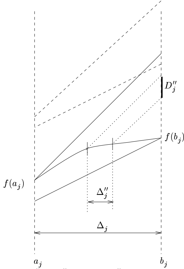
Fig. 2: The bijection between \Delta_j'' and D_j'' . The size of \Delta_j'' is taken here symbolically. See Fig. 3 for a realistic arrangement.
